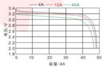
Discharge curves at room temperature
